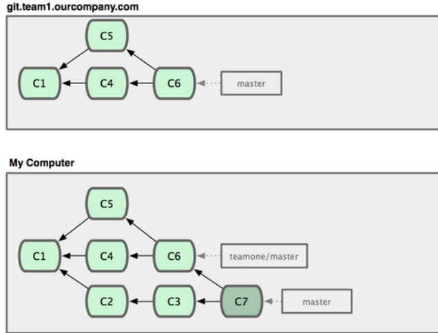
Figure 3.37: Fetch more commits, and merge them into your work.
