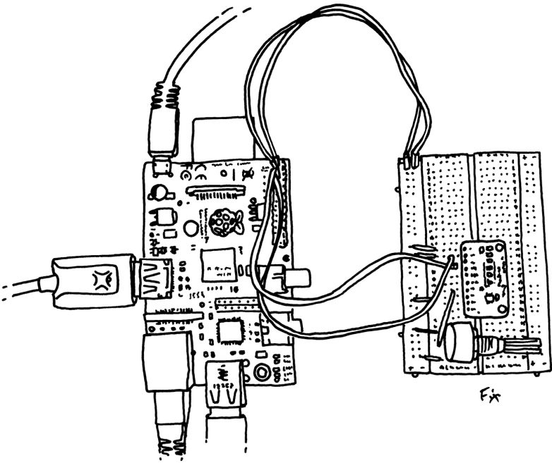
Figure C-2. Using the ADS1015 to connect a potentiometer to the Raspberry Pi
