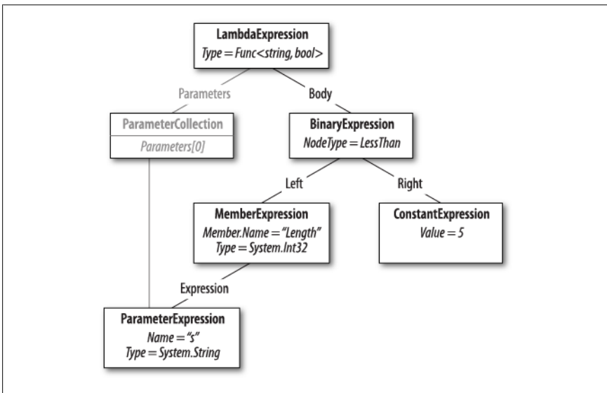
Figure 8-11. Expression tree
