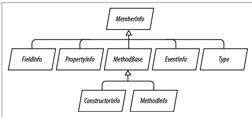
Figure 19-1. Member types
