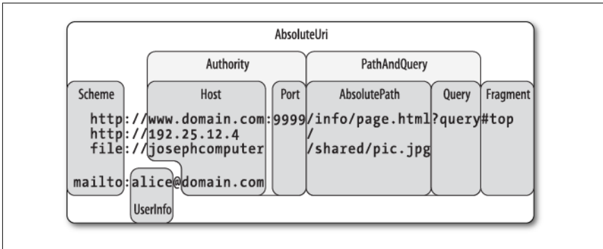
Figure 16-2. URI properties
