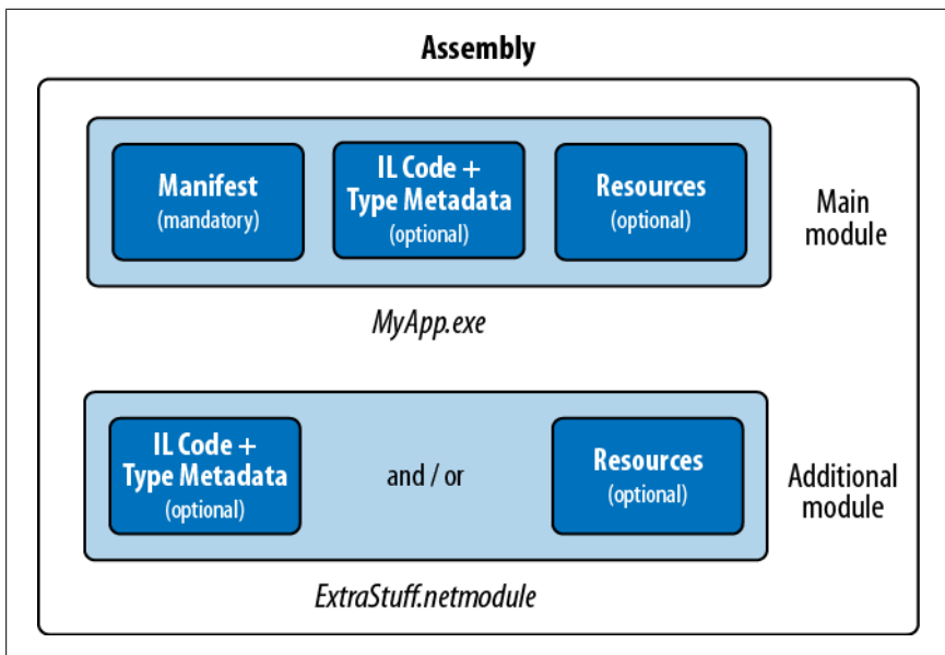
Figure 18-2. Multifile assembly
