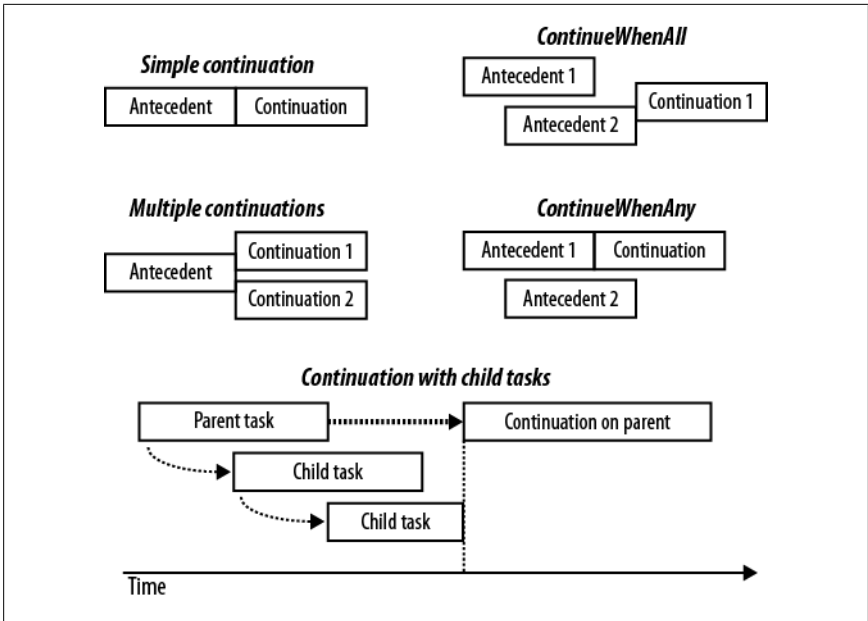
Figure 23-5. Continuations
