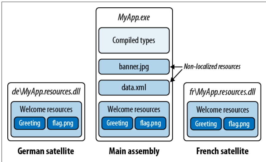
Figure 18-4. Resources
