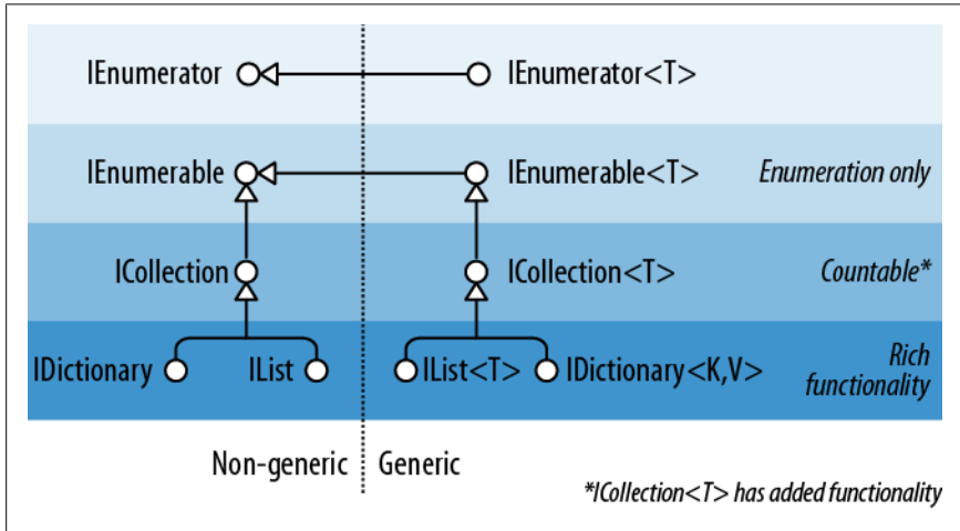
Figure 7-1. Collection interfaces
