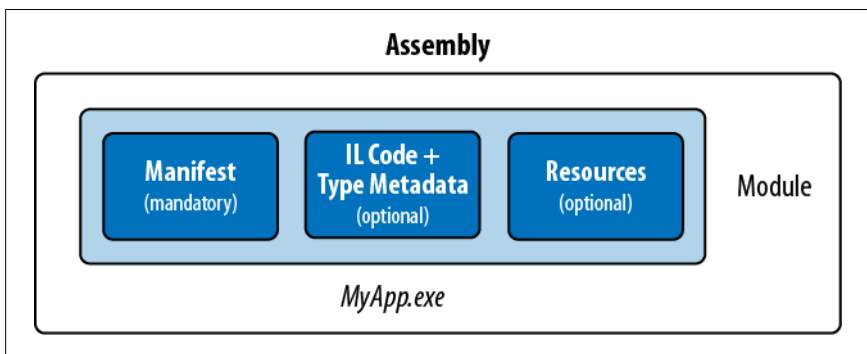
Figure 18-1. Single-file assembly
