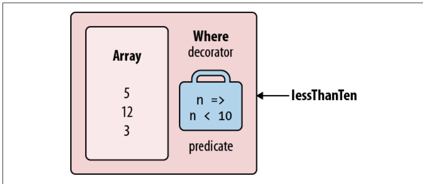
Figure 8-3. Decorator sequence
