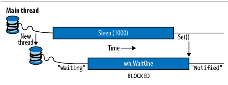
Figure 22-1. Signaling with an EventWaitHandle
